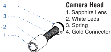
Figure 1. Camera Head
